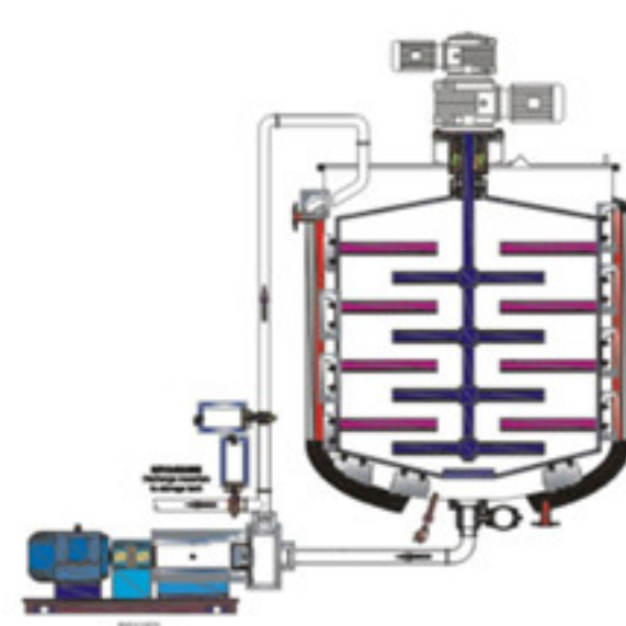
Double way mixing external homogenizer
