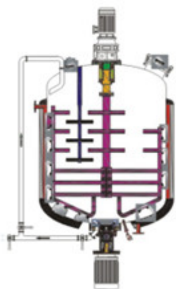
Single way mixing internal external
