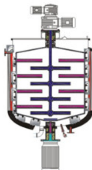
Double way mixing internal circulation
