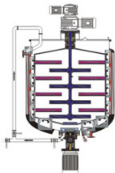
Double way mixing internal external
