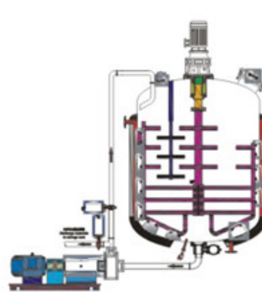
Single way mixing external homogenizer
