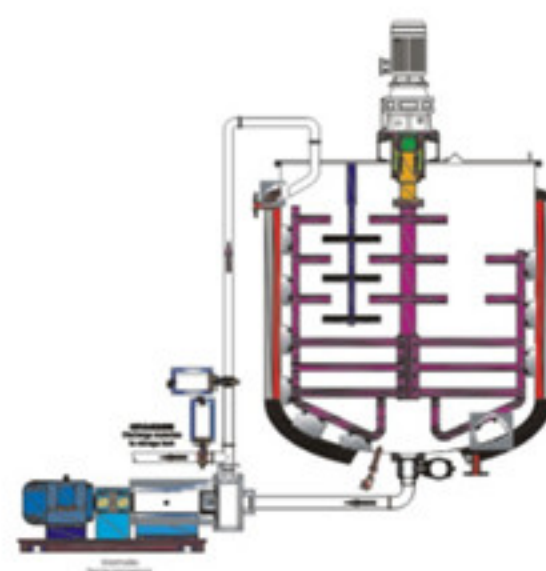
Single way mixing external homogenizer
