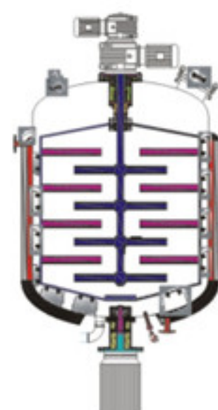
Double way mixing internal circulation
