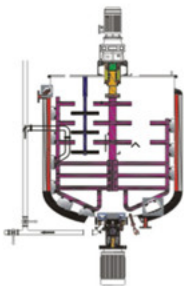
Single way mixing internal external
