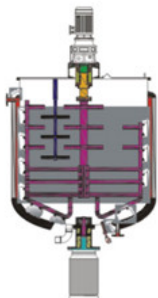
Single way mixing internal circulation
